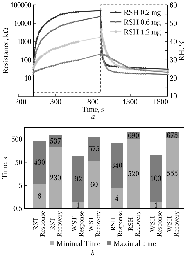
Fig. 7. The response and recovery curves (a) and minimum/maximum values of response and recovery times (b) for resistive humidity sensors based on NC
