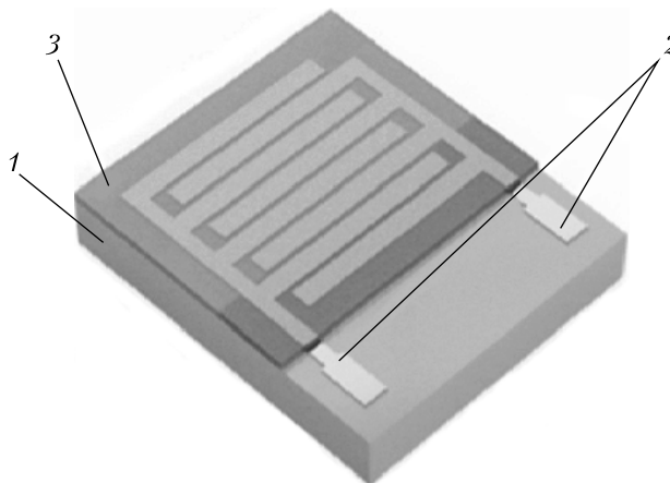
Fig. 1. Structure of a resistive humidity sensor based on NC: 1 – glass-ceramic substrate; 2 – Ni electrodes; 3 – NC film
